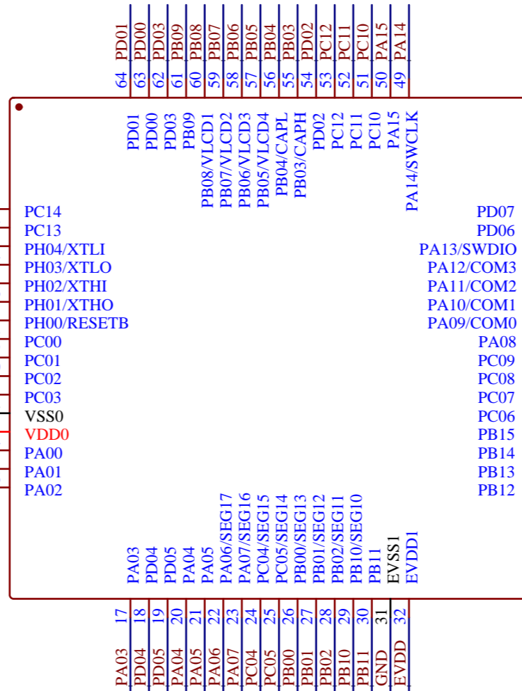
U1 BAT32G127GH64FB
